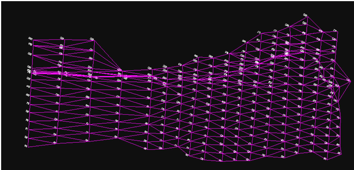
Figure E-1. TIN/DTM of surveyed cross-sections showing 18 cross-sections spaced at 50 ft and 100 ft C/C
