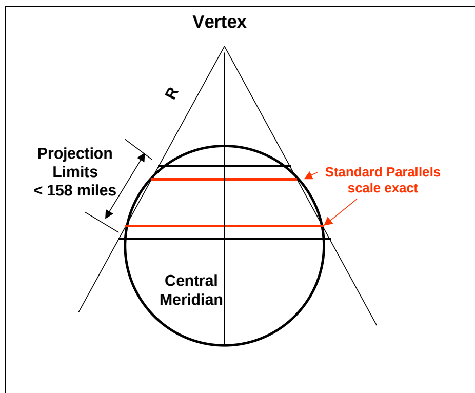
Figure 5-7. Lambert Projection
