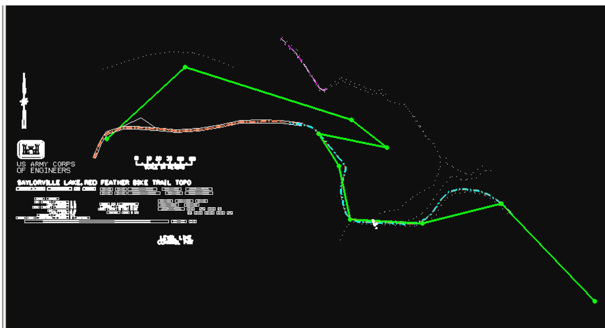
Figure F-3. Primary control traverse (in green) used for controlling topographic mapping of site
