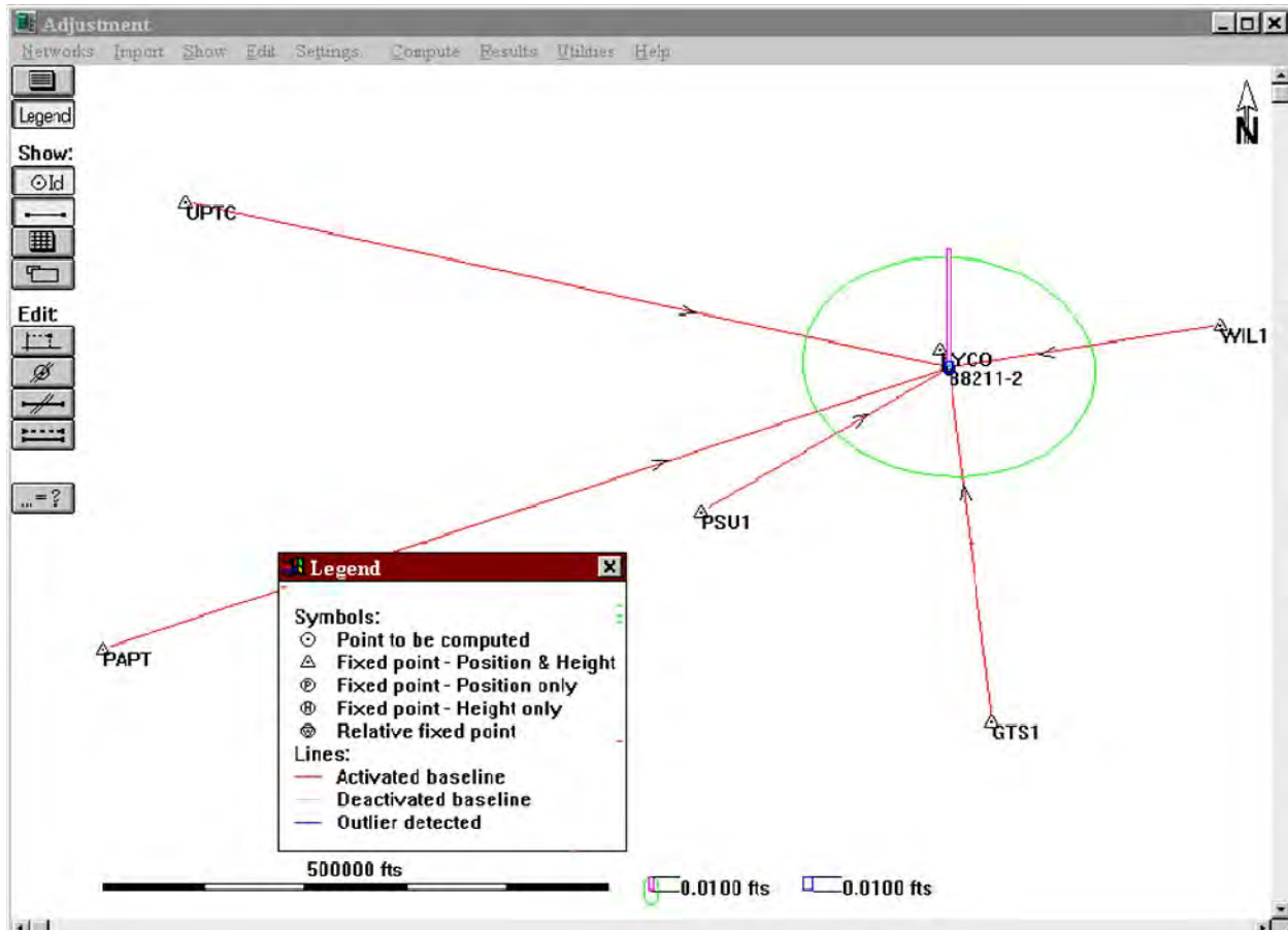
Figure 6-8. Connections to multiple CORS stations to adjust coordinates of a remote point (Leica SKI)
