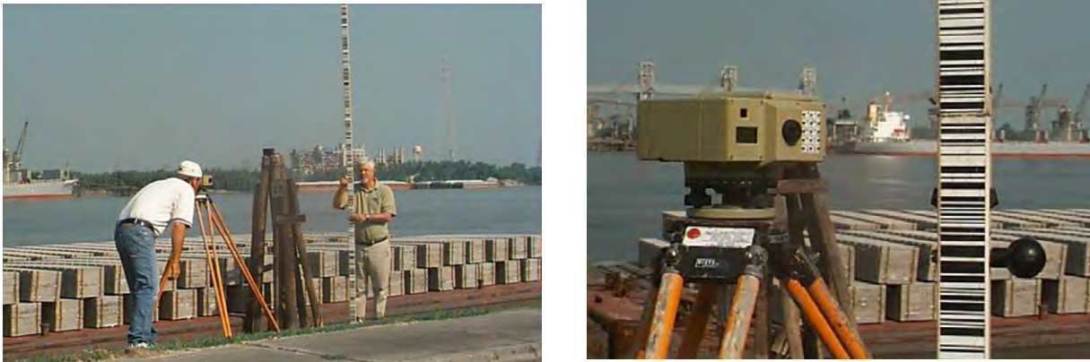
Figure 3-26. Digital Bar Code Level--Wild NA2 (New Orleans District)
