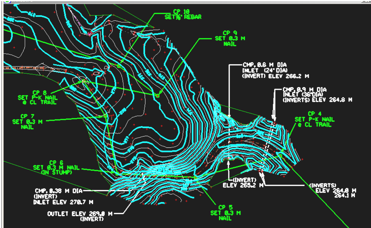
Figure F-4. Eastern portion of survey area
