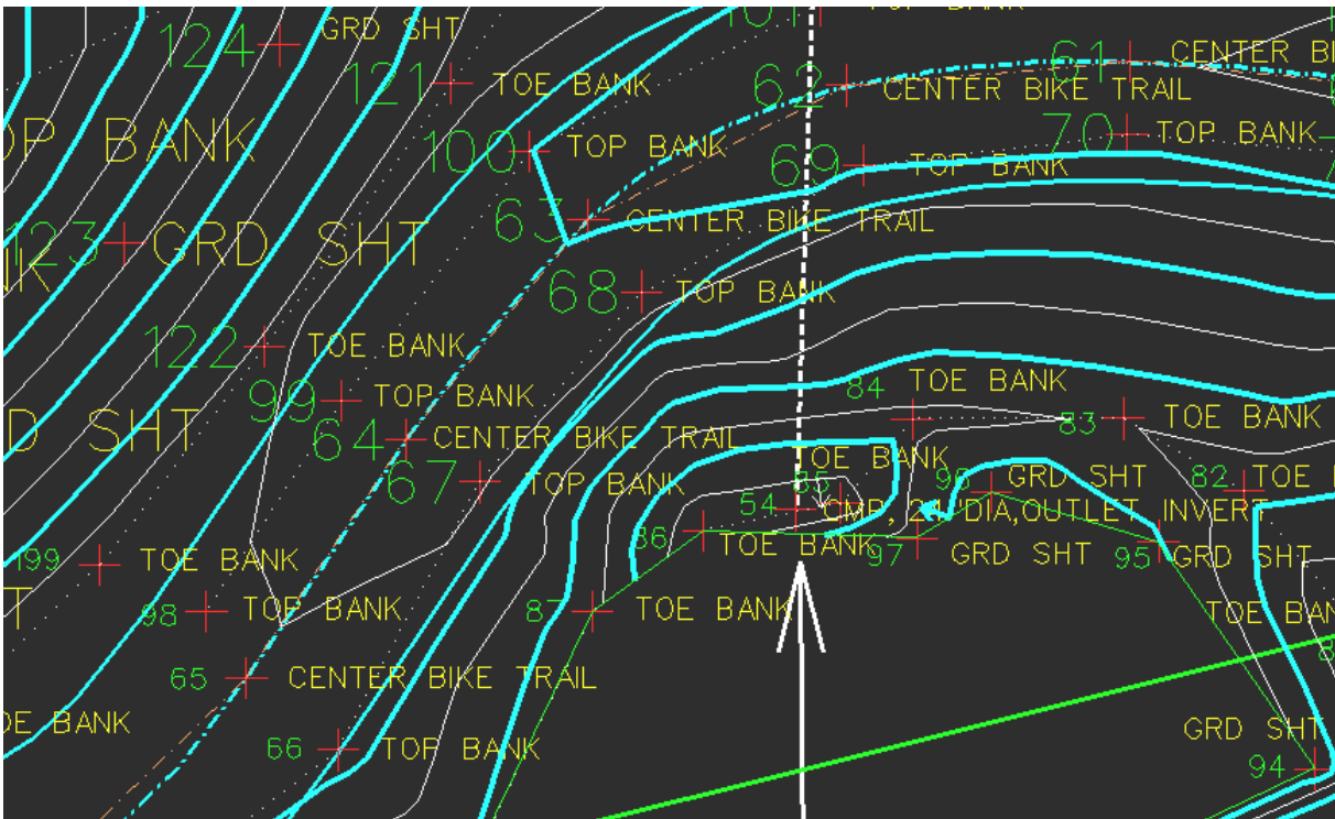
Figure F-6. Screen capture detailing point numbers and descriptors, breaklines, culvert alignment, and trail centerline
