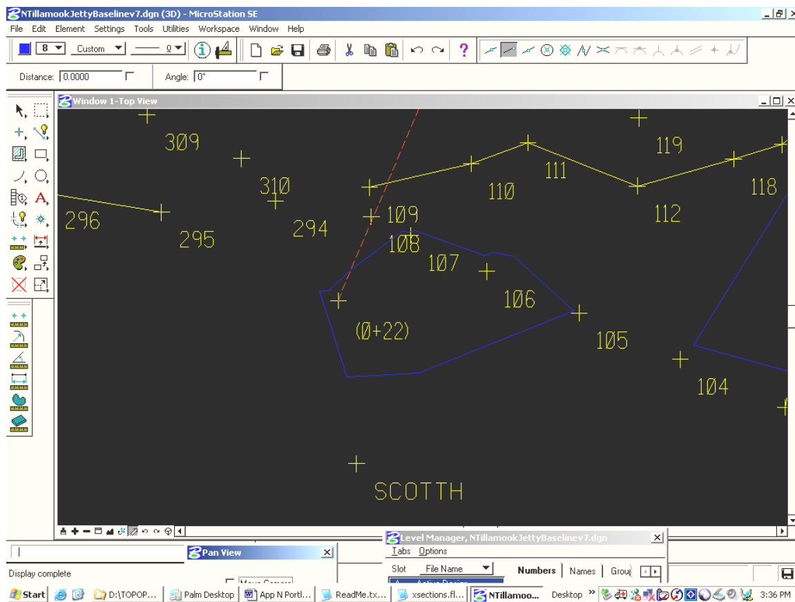
Figure E-2. Total Station occupied Point "0+22"
