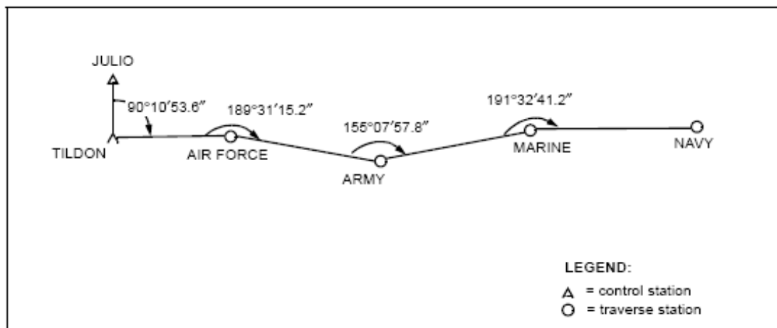
Figure 3-10. Open traverse
