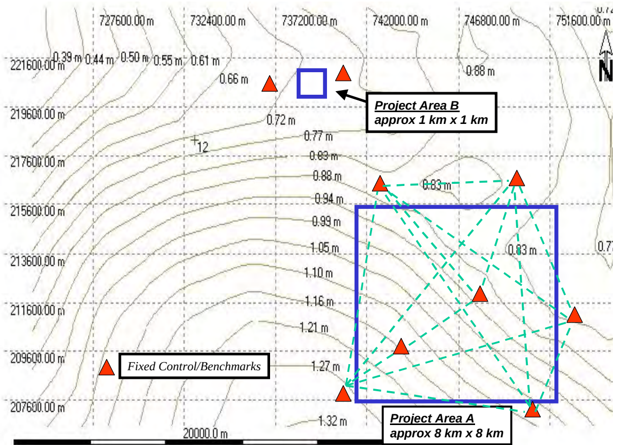
Figure 9-6. Plot of geoid undulation contours over a local survey area (Leica)
